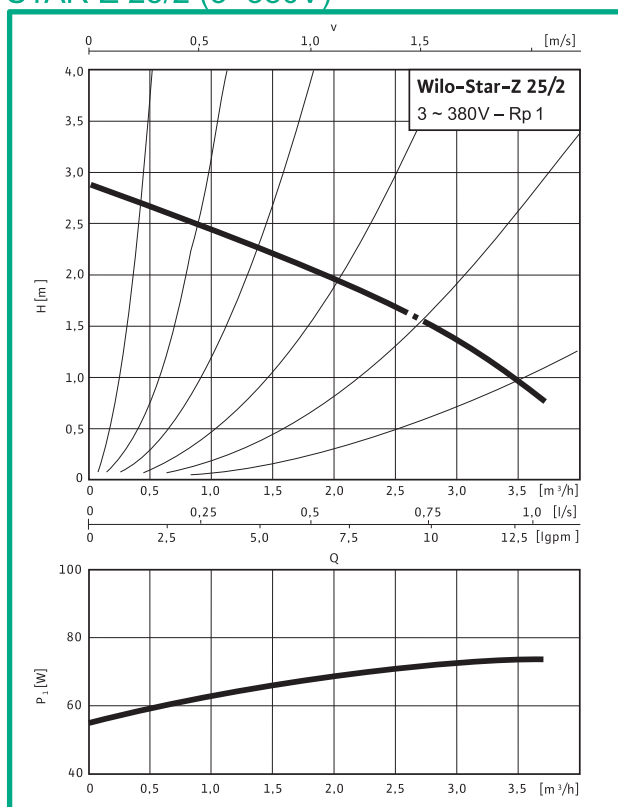
STAR-Z 25/2 (3~380V)
